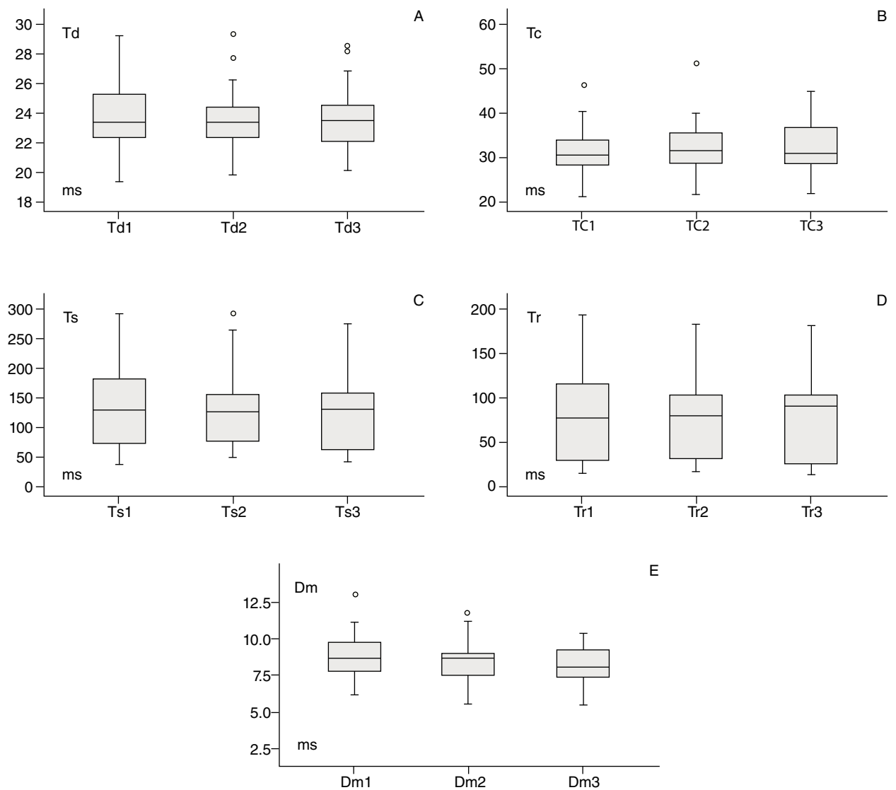
Fig. 2. Distribution of the data obtained from the three measurements (+2, 0, -2) for the five variables assessed by TMG (A: Td; B: Tc; C: Ts; D: Tr; E: Dm). (N = 25). Dm: maximum radial displacement of the muscle belly; Tc: contraction time; Td: reaction time; Tr: relaxation time; Ts: contraction sustain time.
